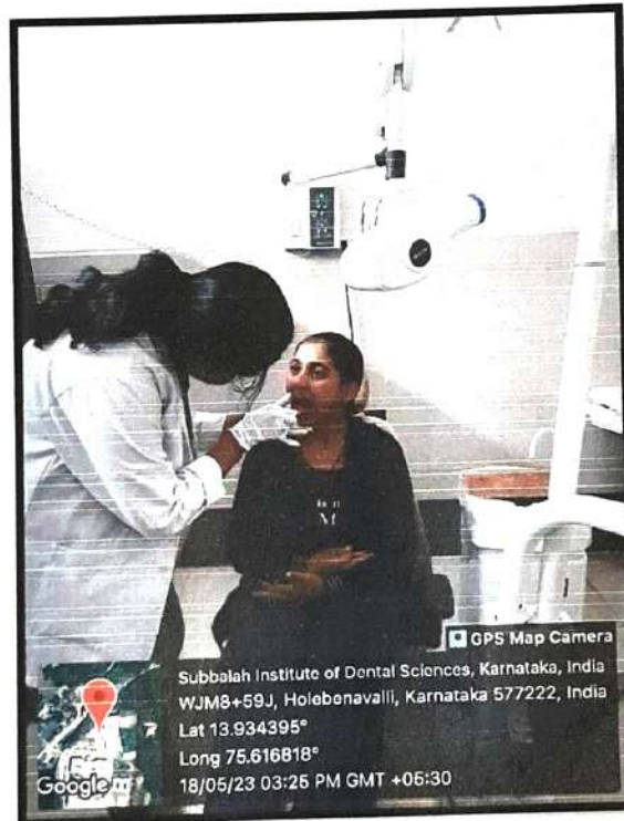
IOPAR technique
