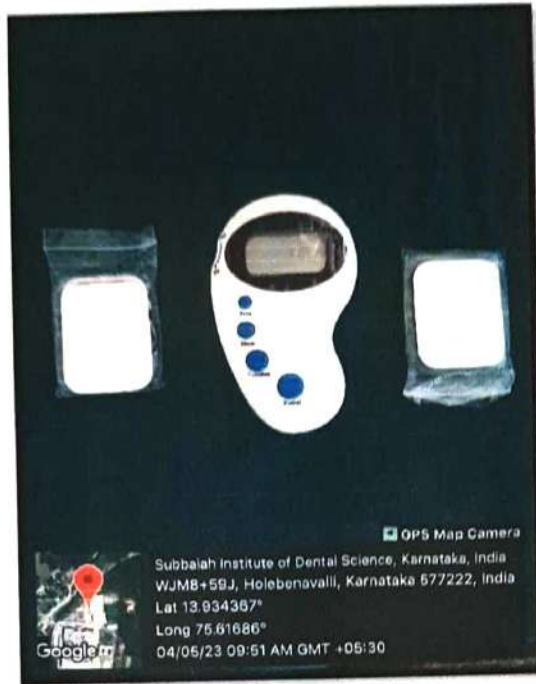
Transcutaneous Electrical Nerve Stimulation machine (TENS)
